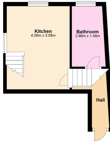
Basement
