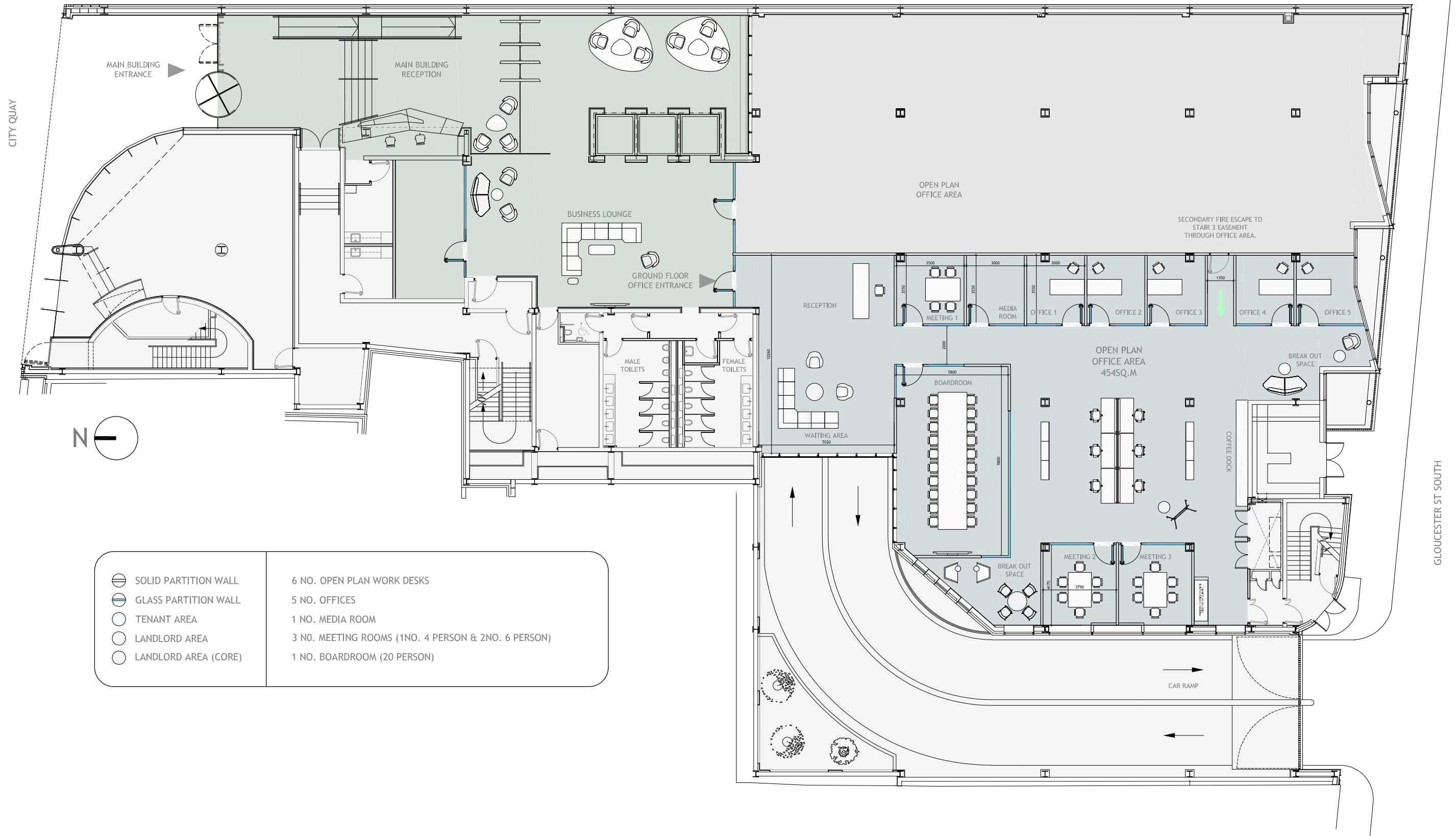
24-26 CITY QUAY GROUND FLOOR PLAN
