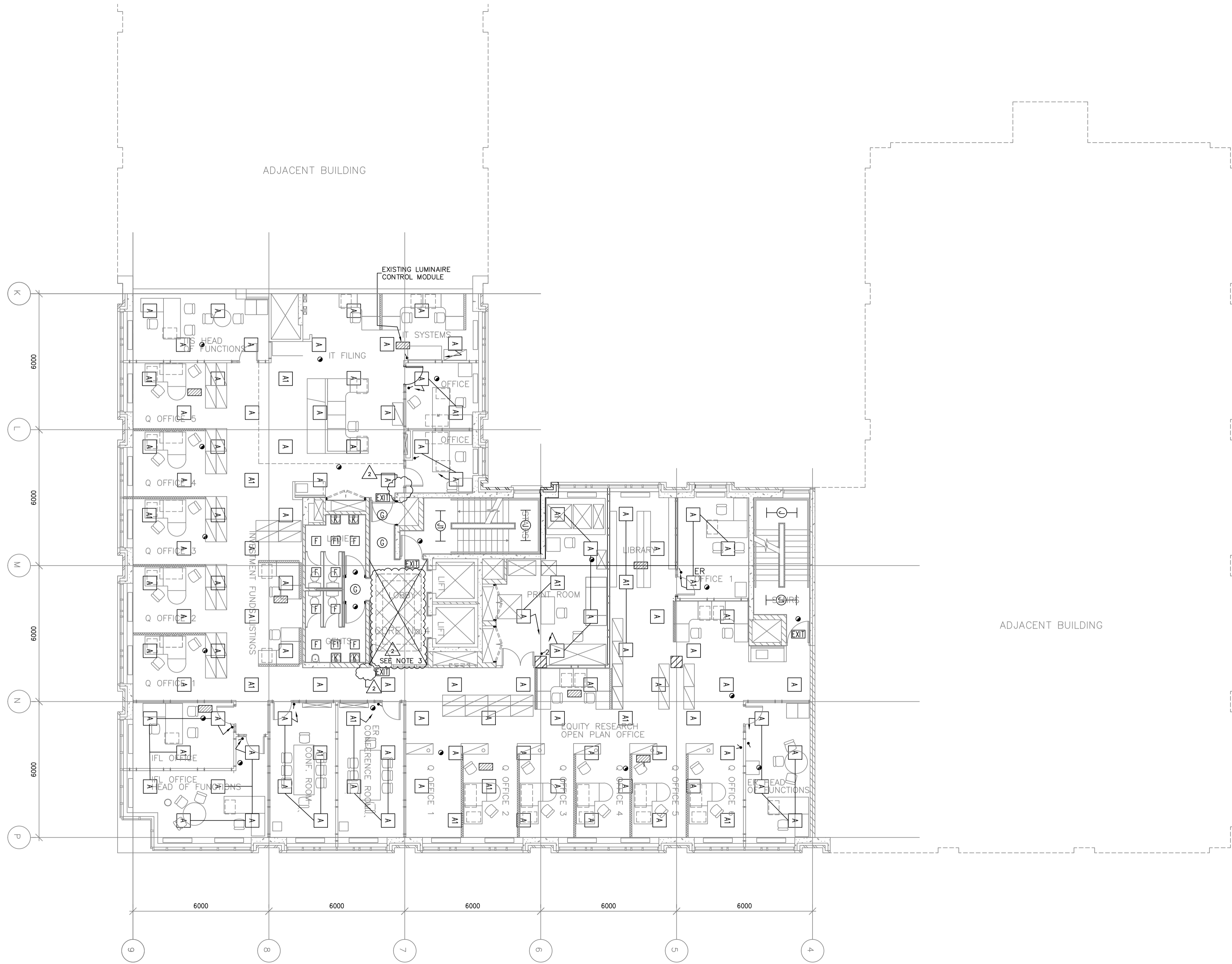
SECOND FLOOR PLAN SCALE 1:100
